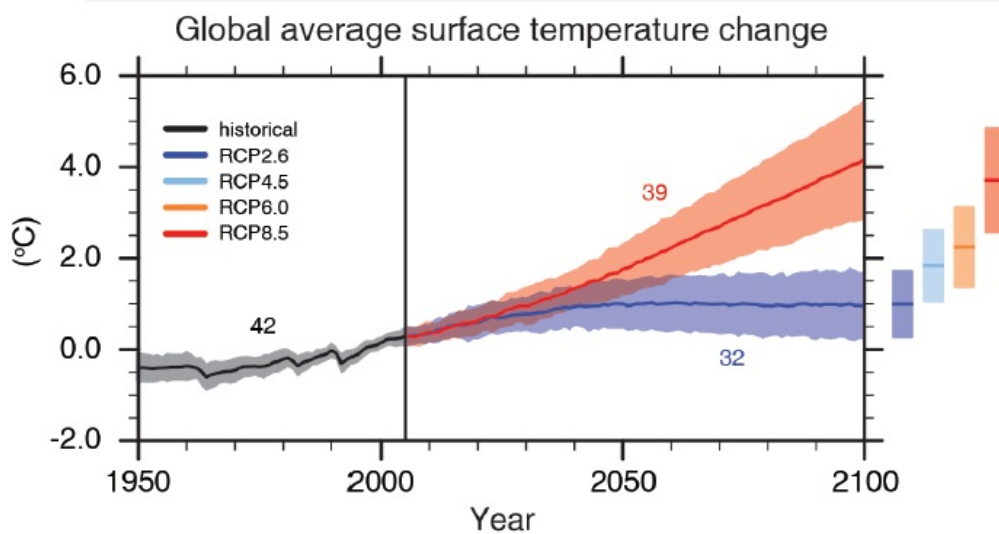
Figure 7: Projected global temperature changes over the rest of the century
